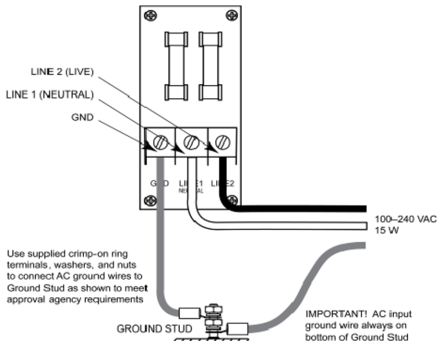
Figure 2-6. AC Power Connections
