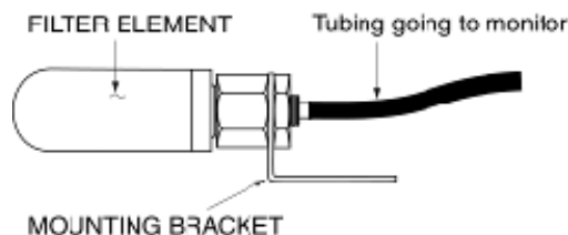
Figure 2-3. Termination Filter (P/N 3015-3420)
