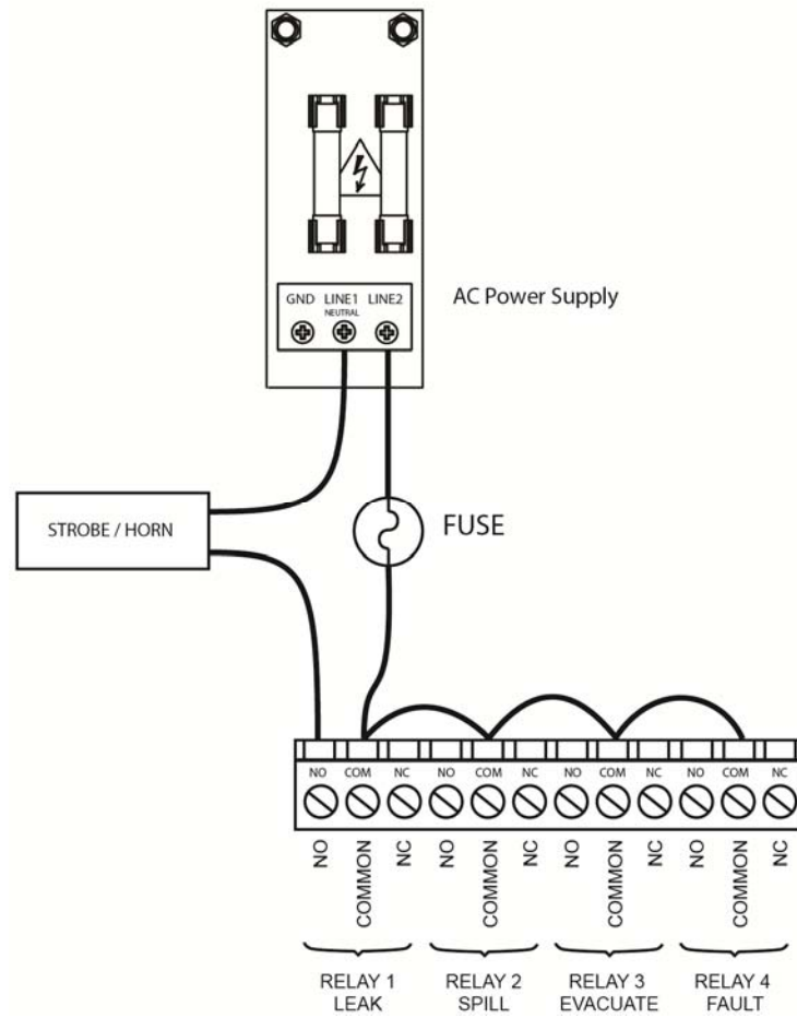
Figure 2-8. Typical AC External Alarm Relay 1 Wiring
