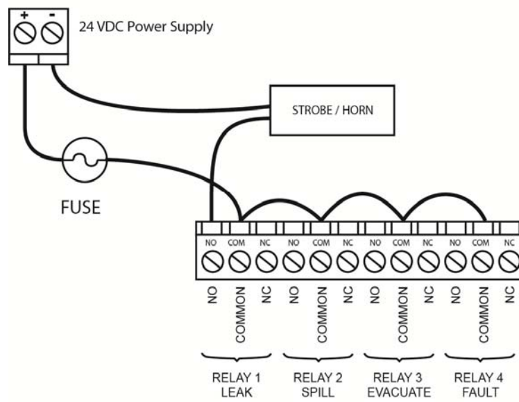
Figure 2-9. Typical DC External Alarm Relay 1 Wiring
