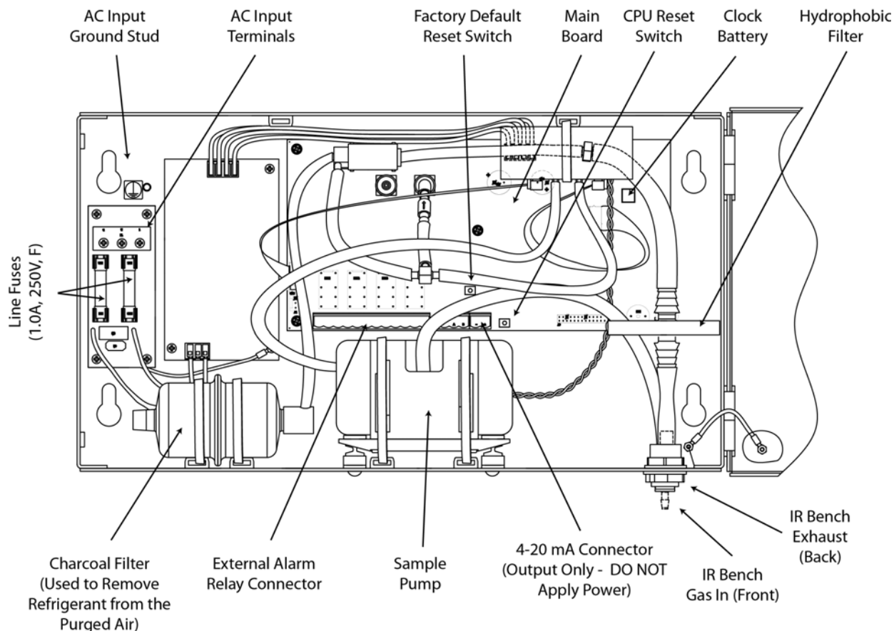
Figure 2-4. Interior Assembly of the Single Zone Halogen Gas Monitor
