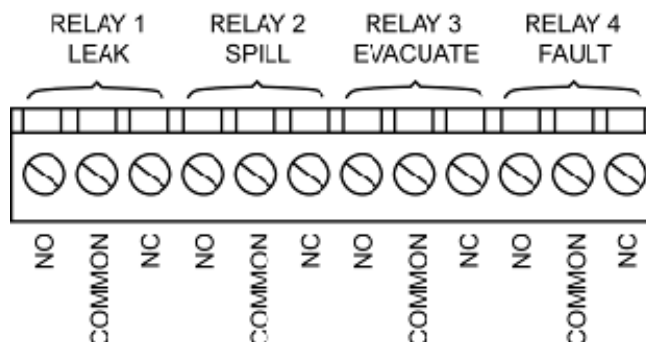
Figure 2-7. External Alarm Relay Connector
