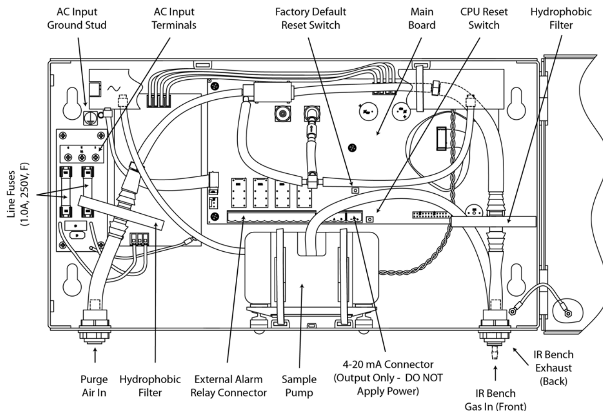
Figure 2-5. Interior Assembly of the Single Zone Ammonia Gas Monitor
